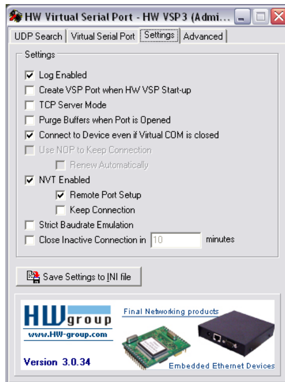
Figure 13: SER2NET configuration
